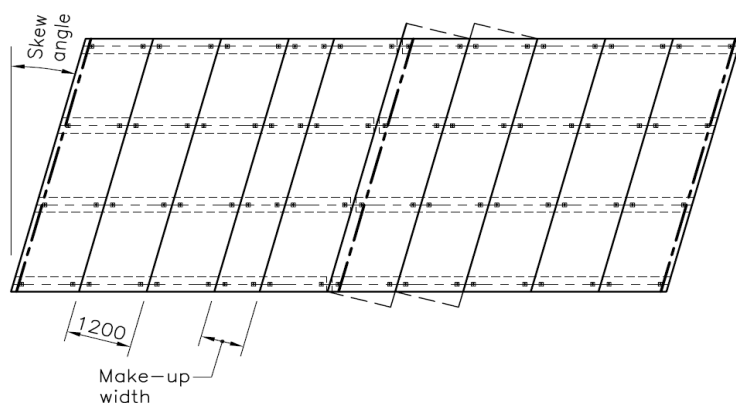
Fig 2: Plan View of Skew Deck
